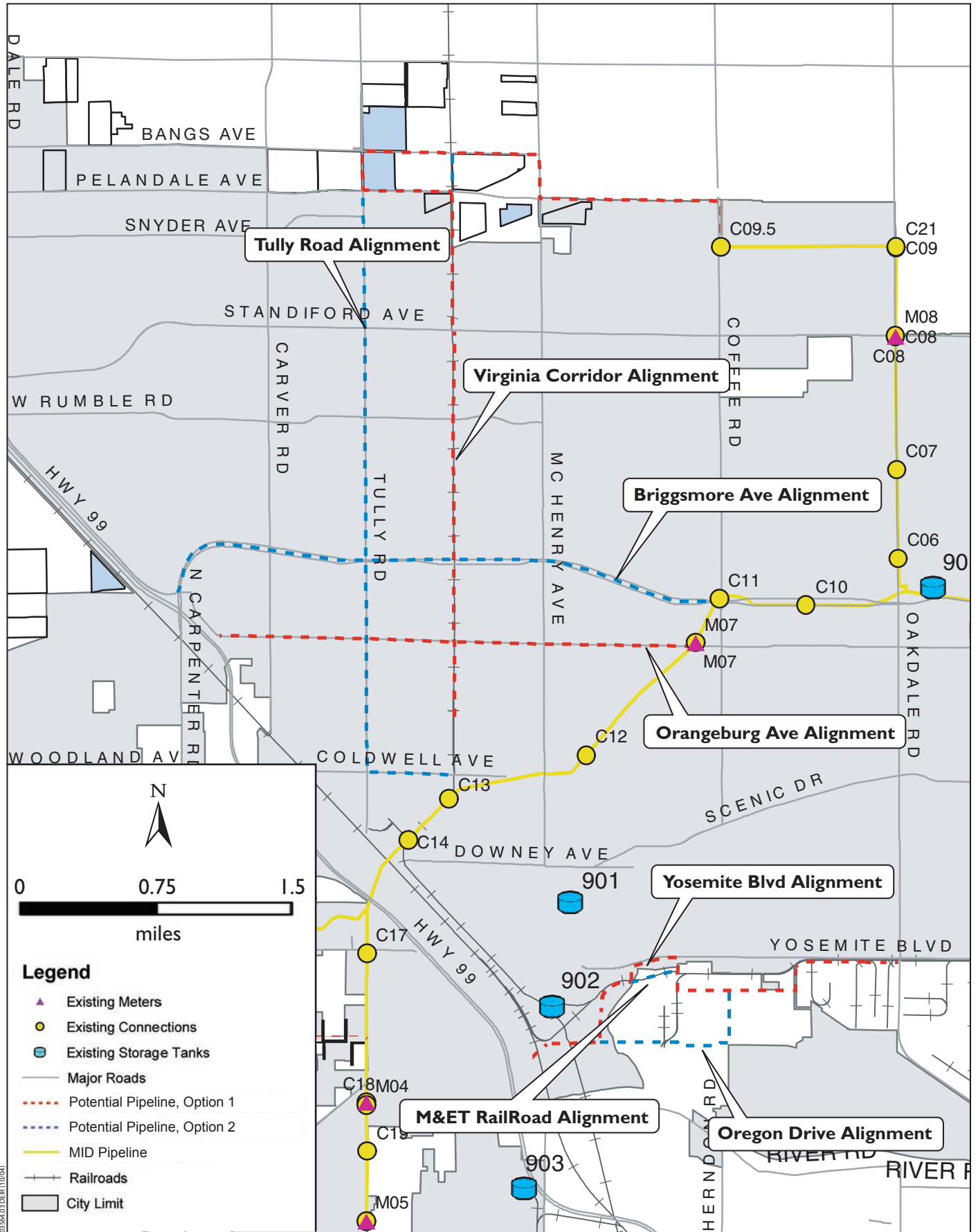
Figure 2-8 Distribution Pipeline
